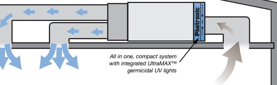
Typical attic HVAC installation
